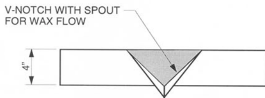
FRONT VIEW OF SHEET METAL WAX PAN
